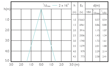
Beam diagram - Master LED PAR30L 40W 30D 840
