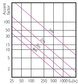
Accent Diagram - Master LED PAR30L 40W 30D 840
