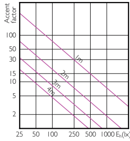
Accent Diagram - Master LED PAR30L 20W 30D 830
