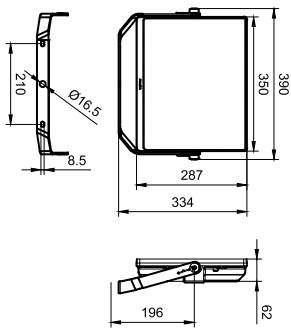
BVP173/174/175/176 Smartbright
