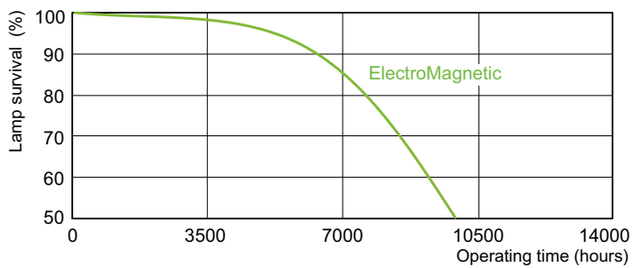
Life Expectancy Diagram - MASTER PL-C 18W/840/2P 1CT/5X10BOX
