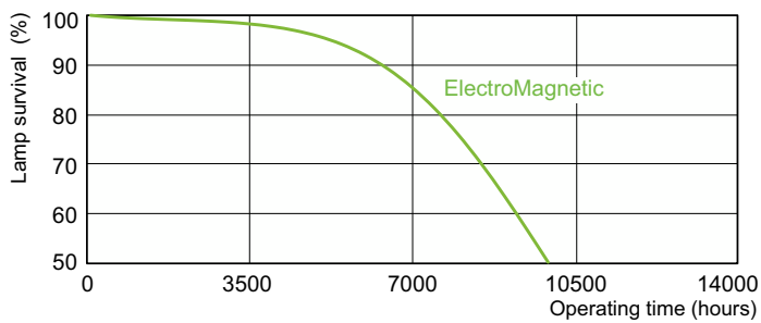
Life Expectancy Diagram - MASTER PL-C 26W/865/2P 1CT/5X10BOX
