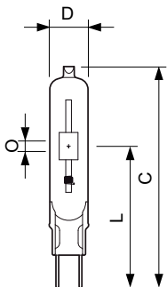
MASTERCcolour CDM-TC 70W/830 G8.5 1CT/12
