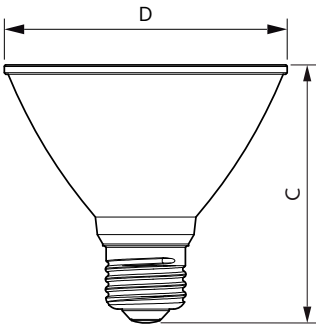
Plastic PAR30s 12-75W 850lm 6500K E26 ND
