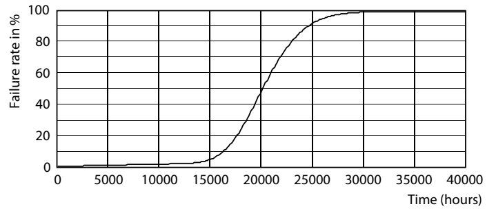
Life Expectancy Diagram - Apex SQ LED 55W 5700K
